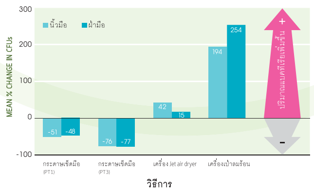
Graph of mean percentage change in numbers of bacterial colony-forming units (CFUs) on all 3 growth media (NA,CLED,MSA) after hand drying using 4 different methods.
