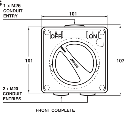
FRONT COMPLETE
